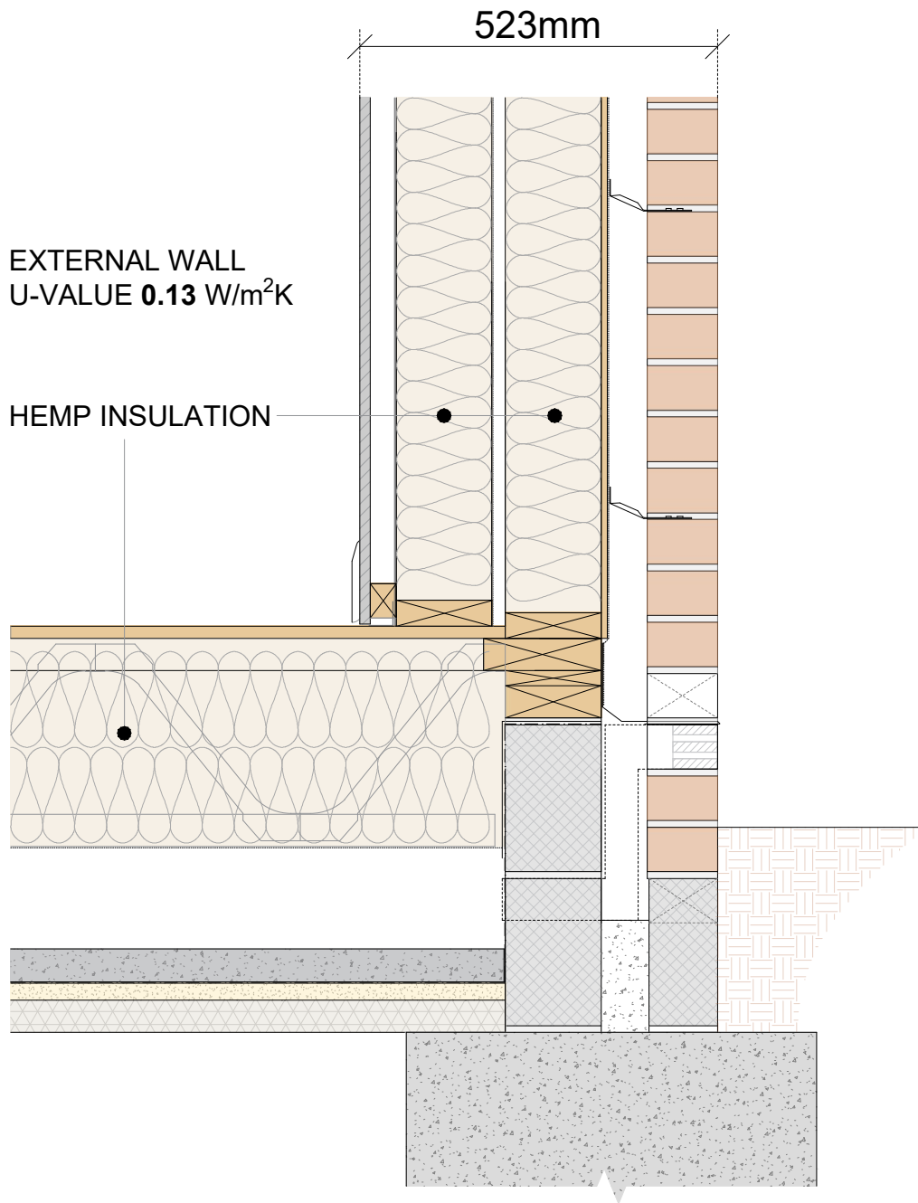
BIO TW MWJ - BRICKWORK 0.13
