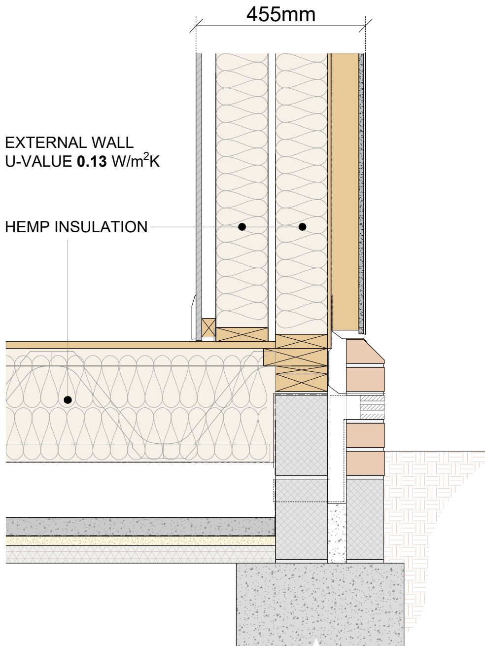
BIO TW MWJ - BRICK PLINTH - RENDER 0.13
