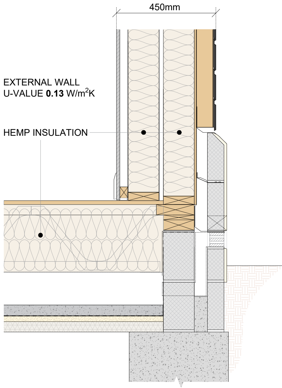
BIO TW MWJ - BLOCK PLINTH - TIMBER CLADDING 0.13
