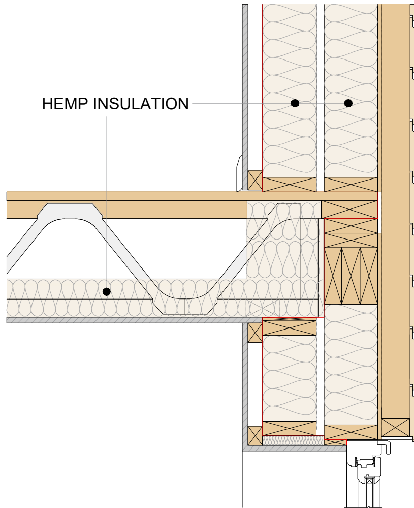
BIO TW IJZ - TIMBER CLADDING
